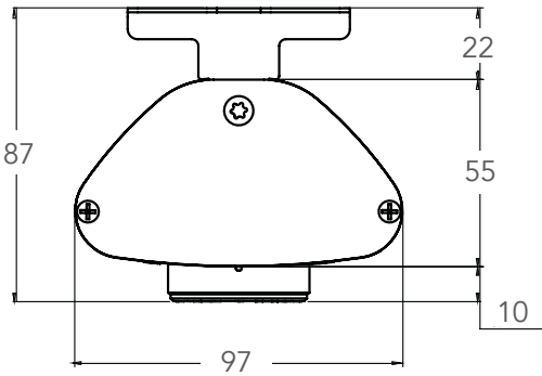
SIDE PROFILE
