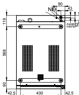
Connection positions in appliance floor
